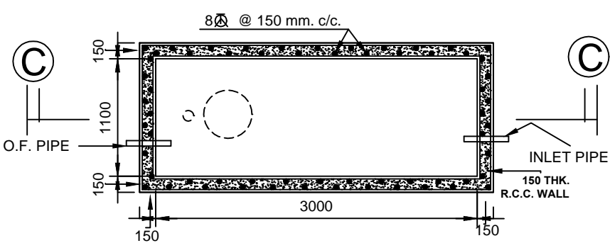
PLAN OF R.C.C. SEMI U/G. WATER RESERVOIR (CAPACITY - 800 GLS.)
