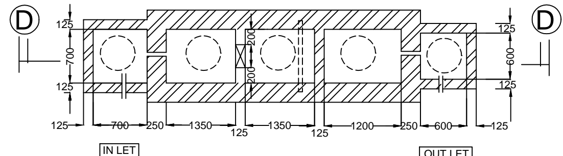
PLAN OF SEPTIC TANK FOR 50 USERS
